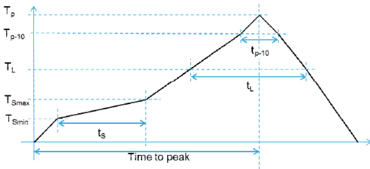
Figure 36. Solder profile
