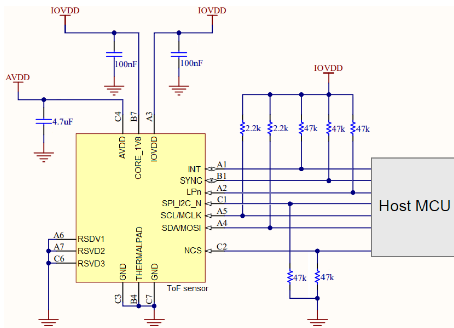
Figure 5. Typical application schematic for I 2 C
