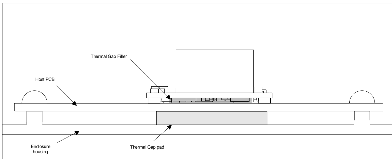
Figure 11: Additional Heatsinking
