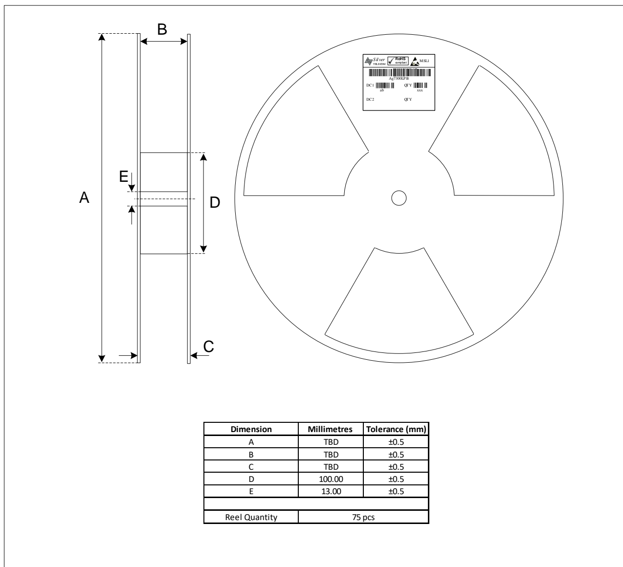
Figure 16: Reel Dimensions
