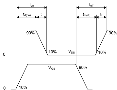
Figure 21. Switching time waveforms
