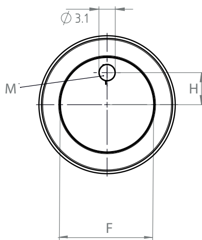
Point illumination(PI)
