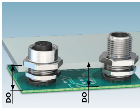
Front mounting, two-piece
