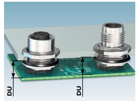
Rear mounting, two-piece
