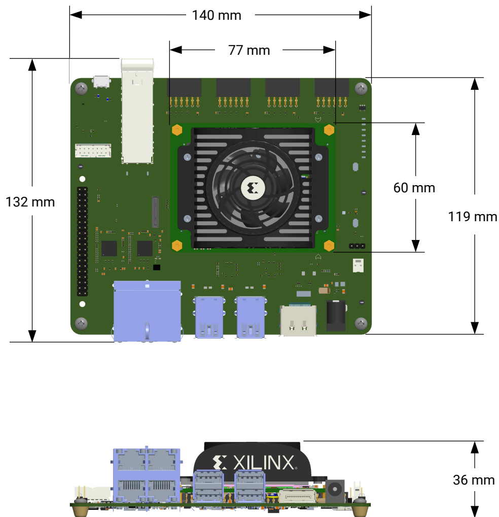
Figure 4: Kria KR260 Robotics Starter Kit Mechanical Dimensions
