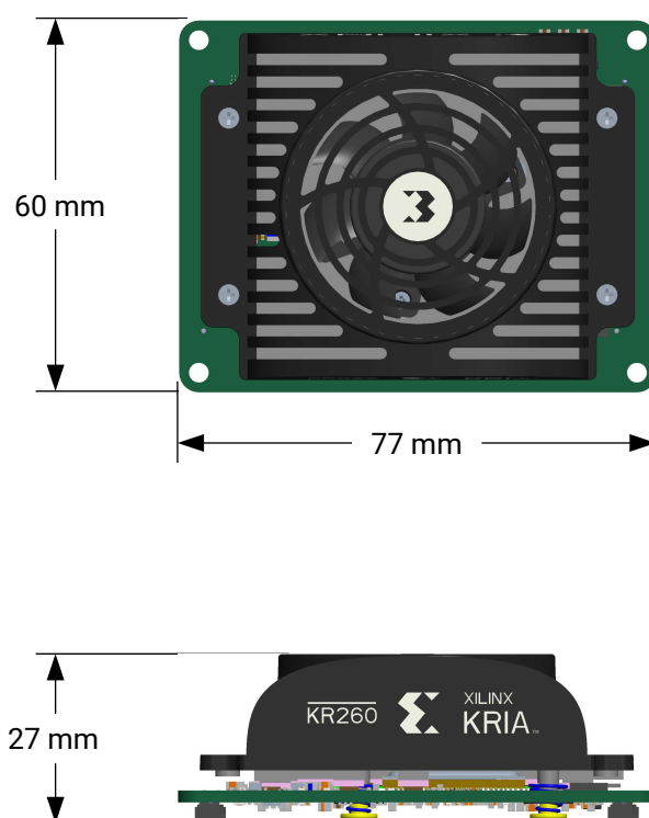
Figure 3: Kria K26 Starter Kit SOM Mechanical Dimensions
