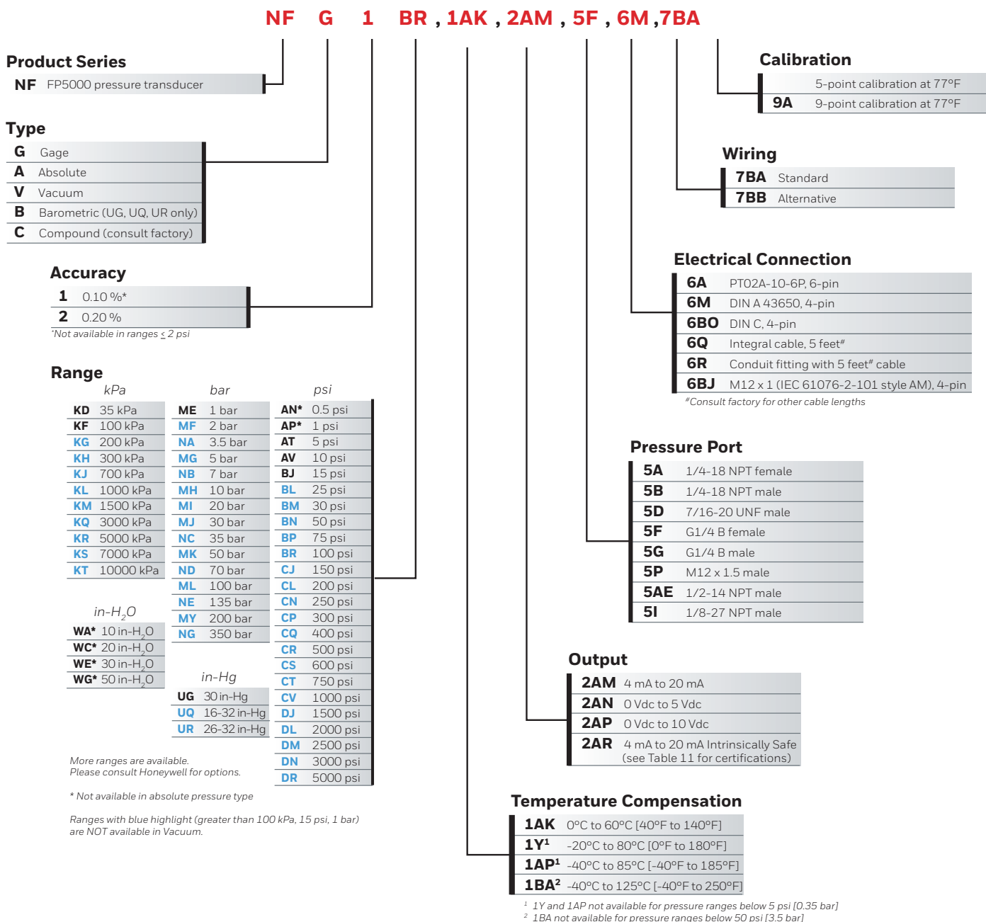
Figure 1. Product Nomenclature
