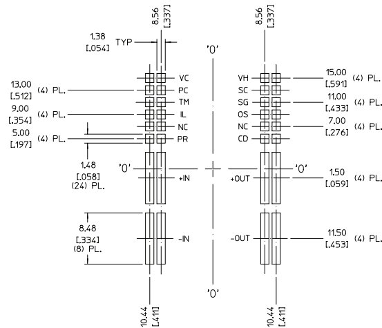
RECOMMENDED LAND PATTERN (COMPONENT SIDE SHOWN)
