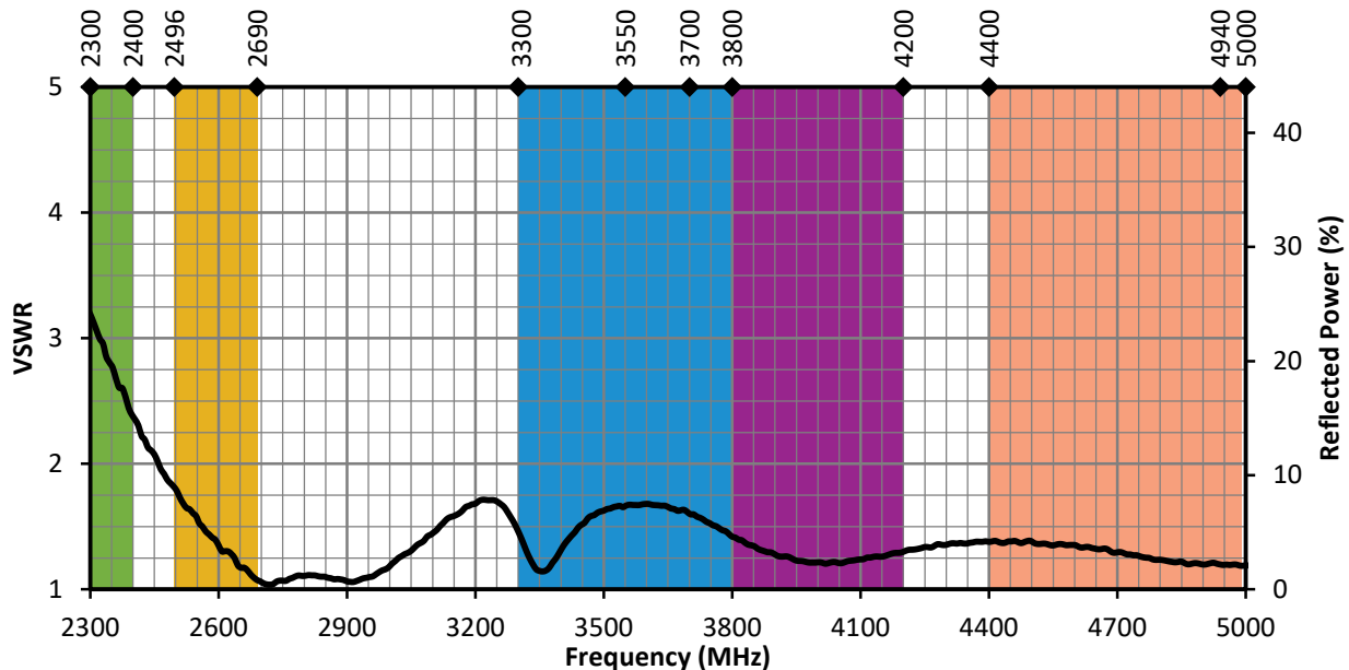
Figure 1. 5GMFPC1 VSWR with Frequency Band Highlights
