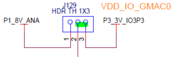
Figure 29. Schematics snapshot showing default position of J129
