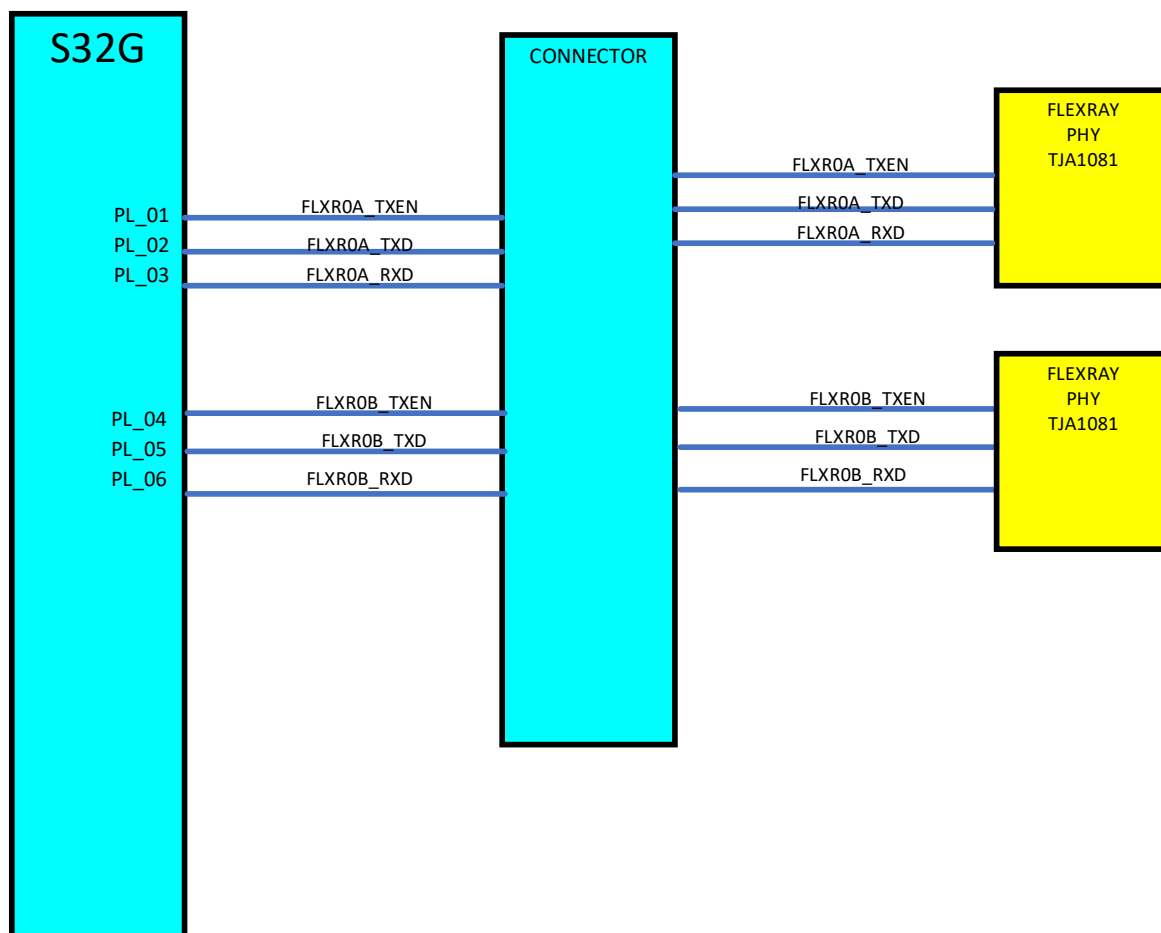
Figure 18. FlexRAY interfacing with S32G-VNP-EVB3
