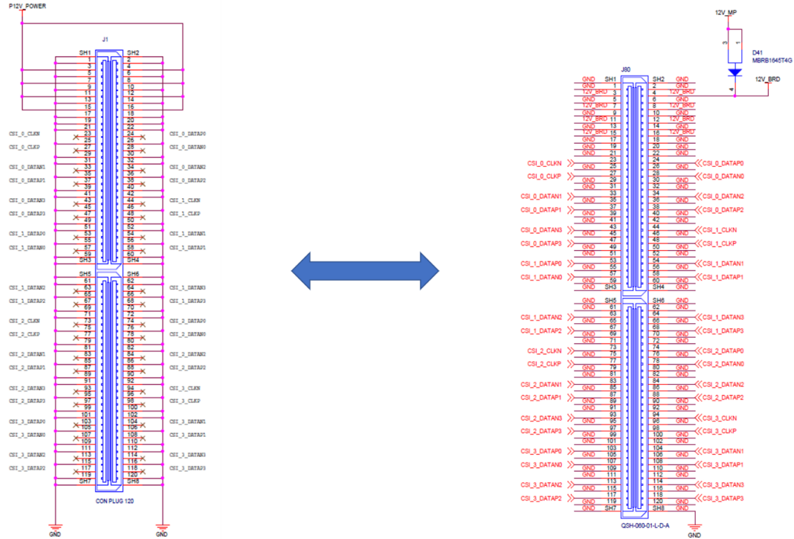
Figure 5. J1<->J80 connection
