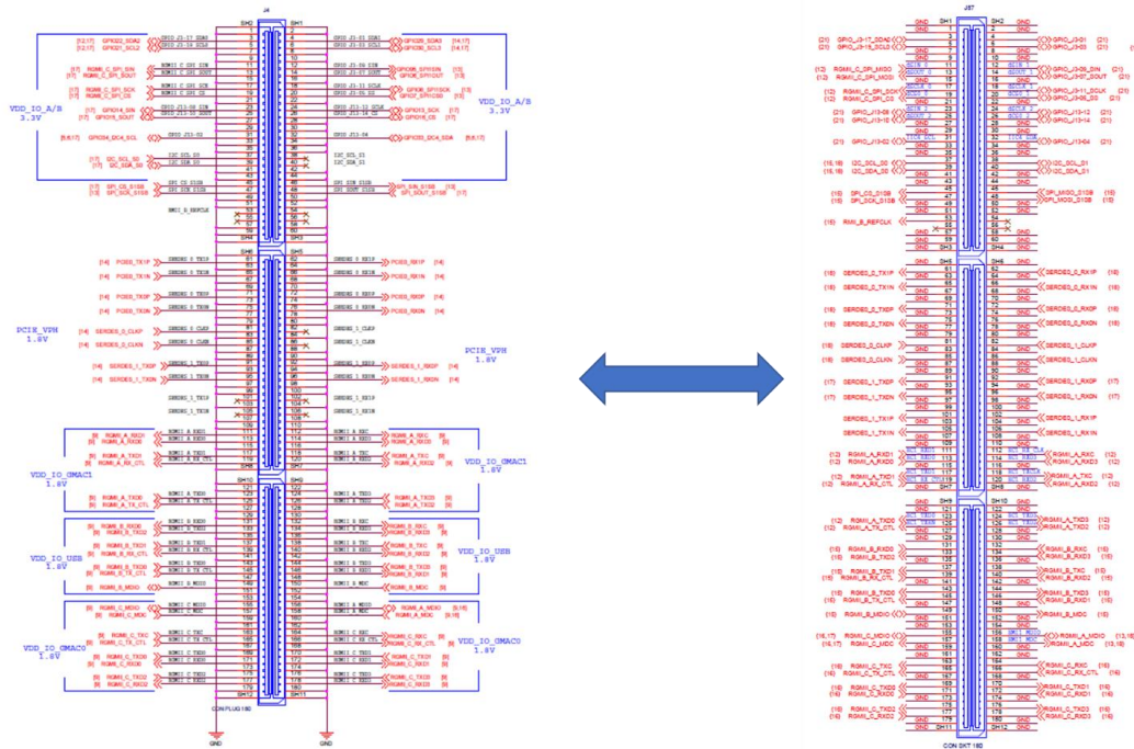
Figure 8. J4&lt;-&gt;J87 connection
