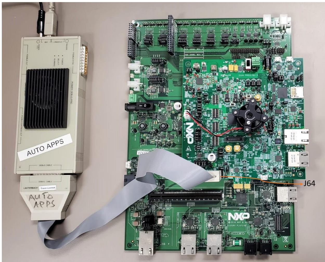
Figure 10. Connecting 20-pin Lauterbach cable on S32G-PROCEVB3-S
