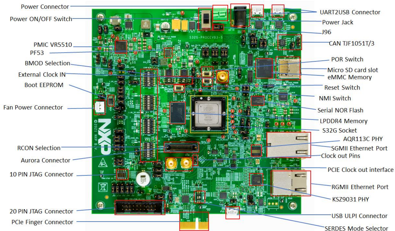
Figure 3. S32G-PROCEVB3-S key areas
