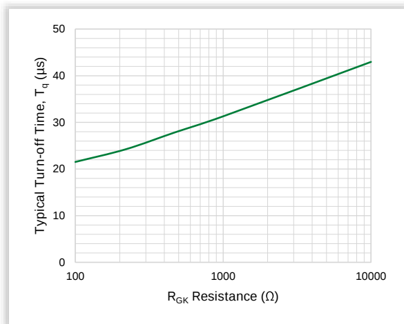
Figure 10. Typical Turn-off Time vs. R_{GK}
