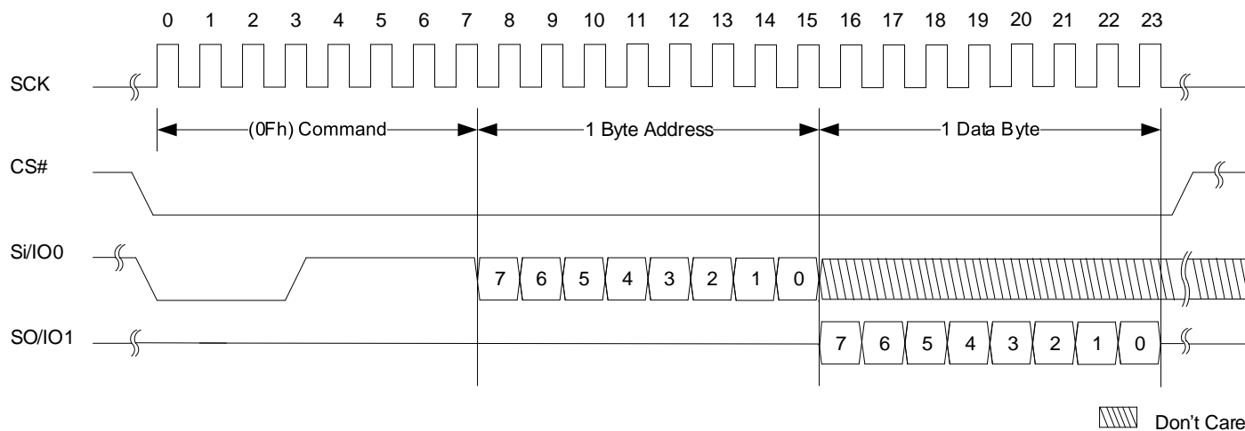
Figure 9. GET FEATURE Timing Diagram
