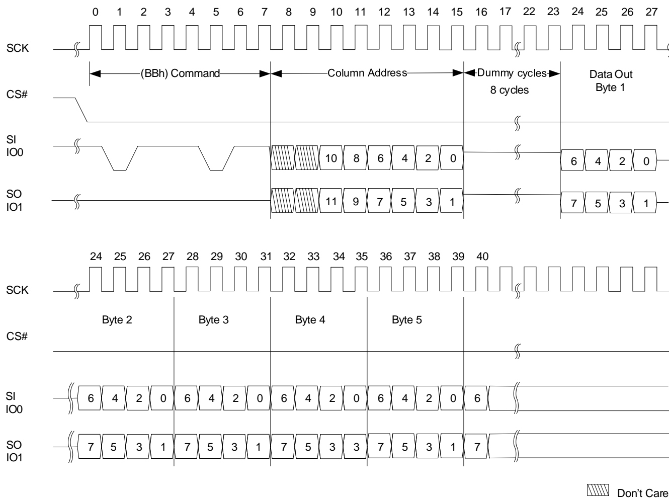
Figure 22. Fast Read Dual IO 2X(BBh) Timing Diagram
