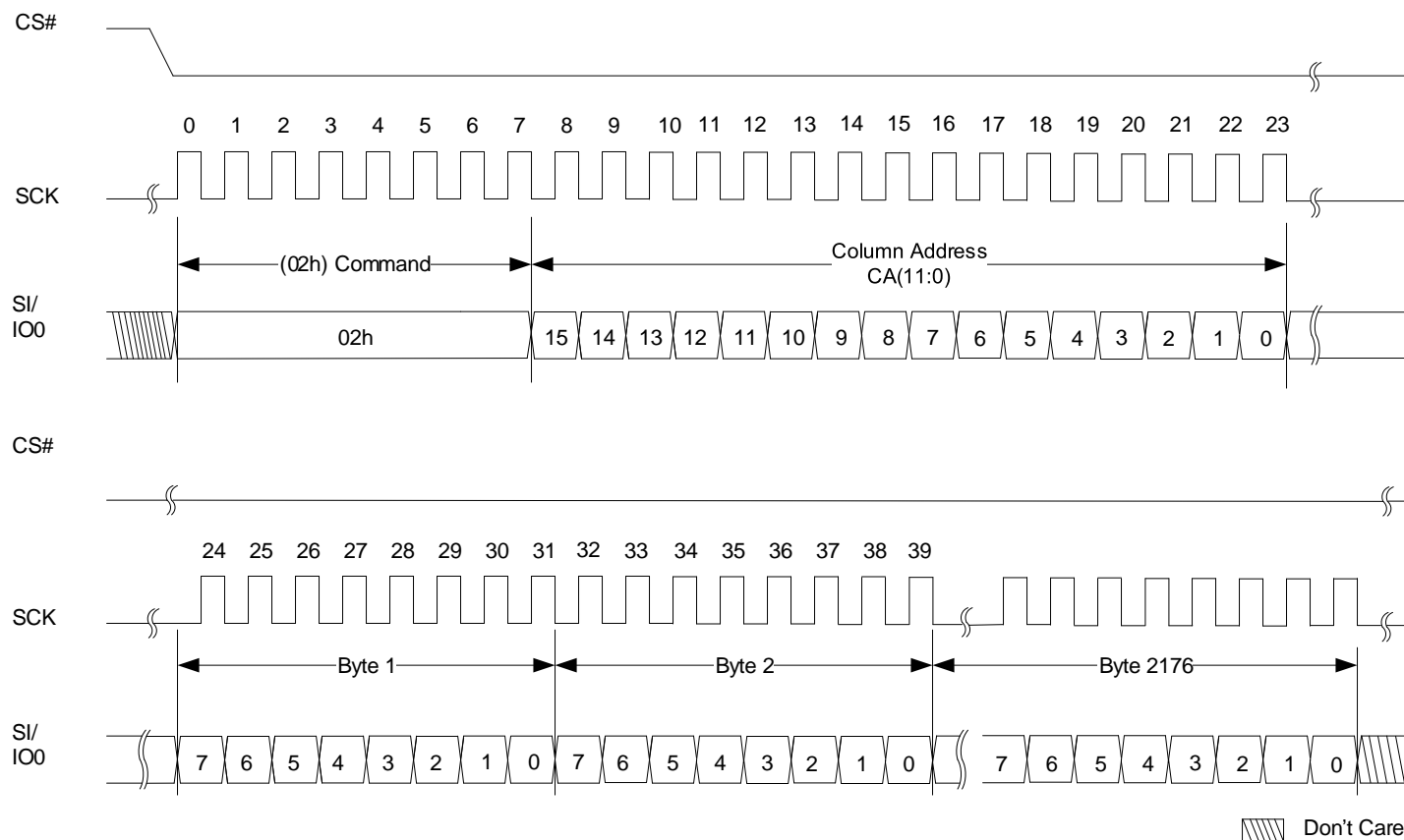
Figure 20. Program Load 1X (02h) and Program Load Random Data 1X Buffer Timing
