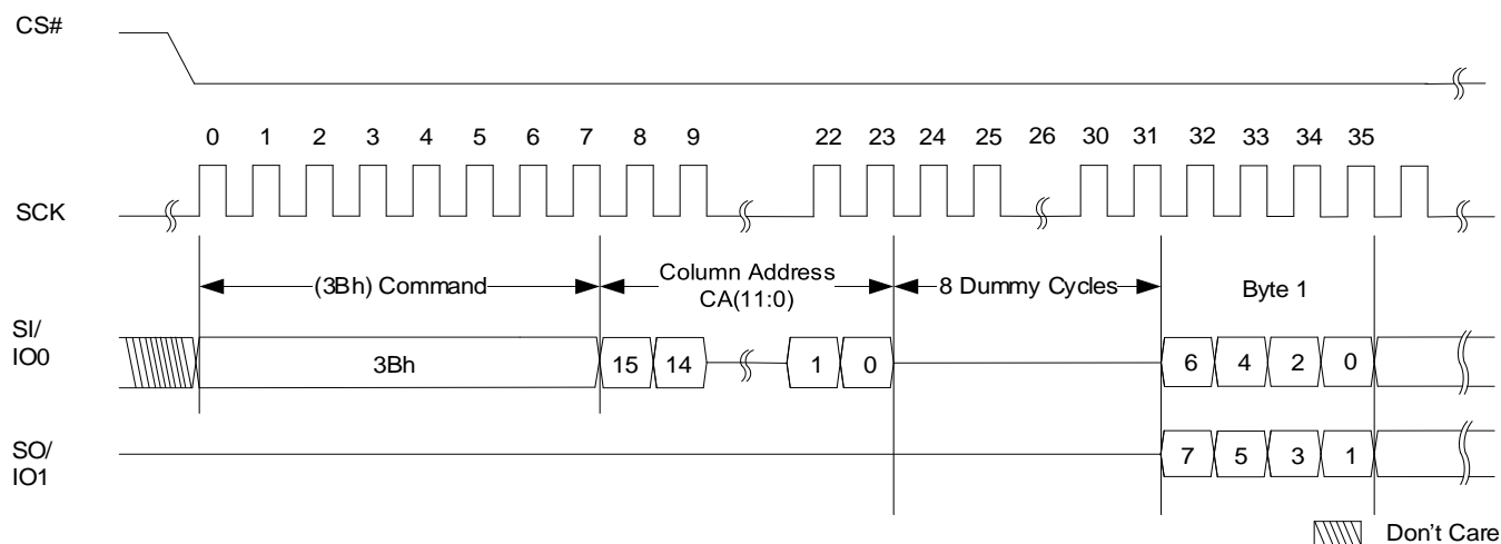
Figure 18. Dual Read Output Buffer 2x (3Bh) Timing
