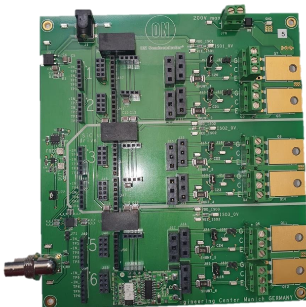
Figure 3.1 SECO-GDBB-GEVB
