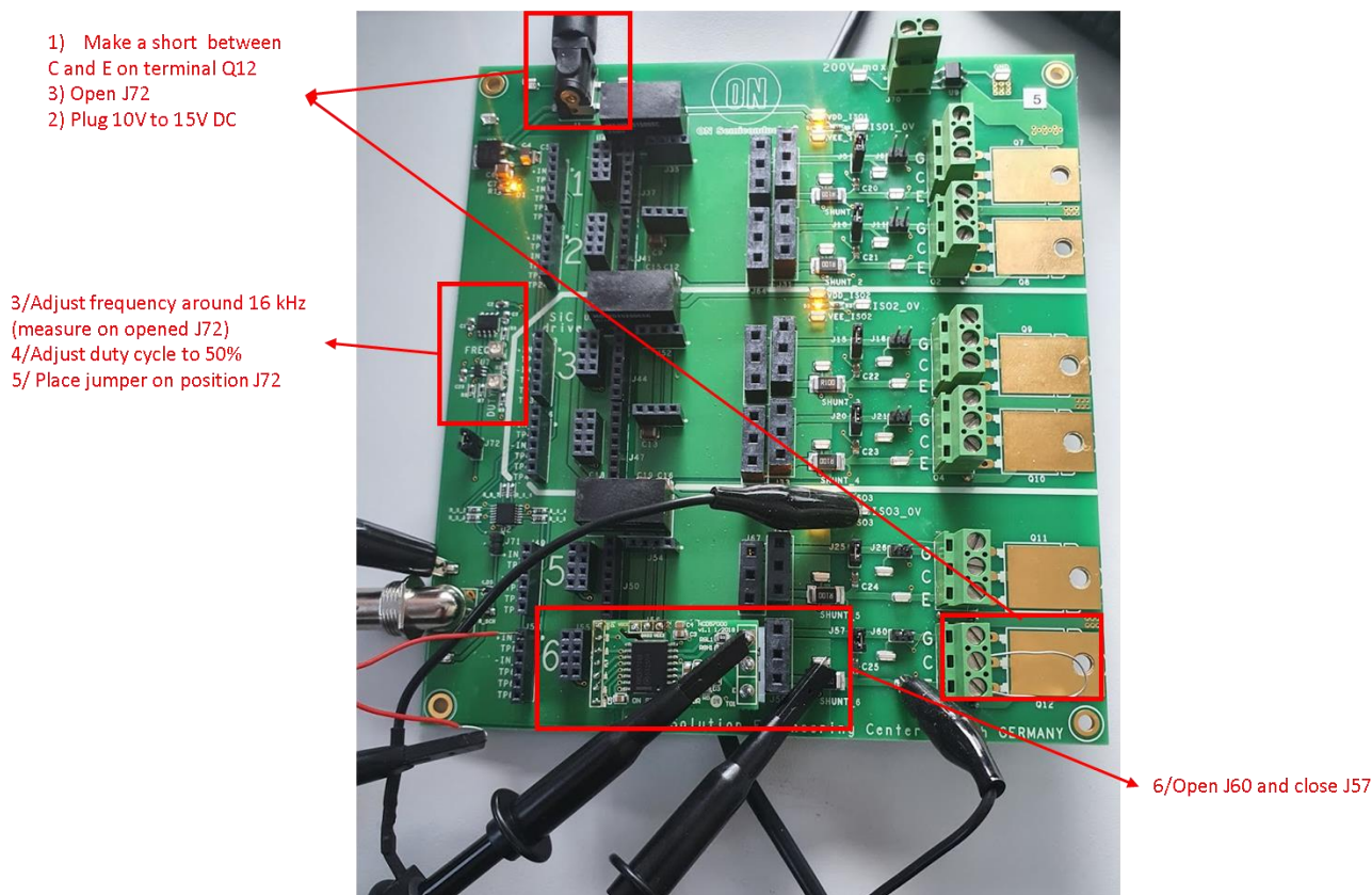
Figure 11. One of examples how to use extended mother board (SECO-GDBB-EVB) for gate drive mini boards testing and evaluating
