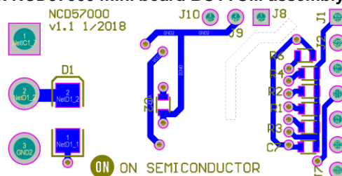
Figure 5. NCD57000 mini board BOTTOM assembly drawing
