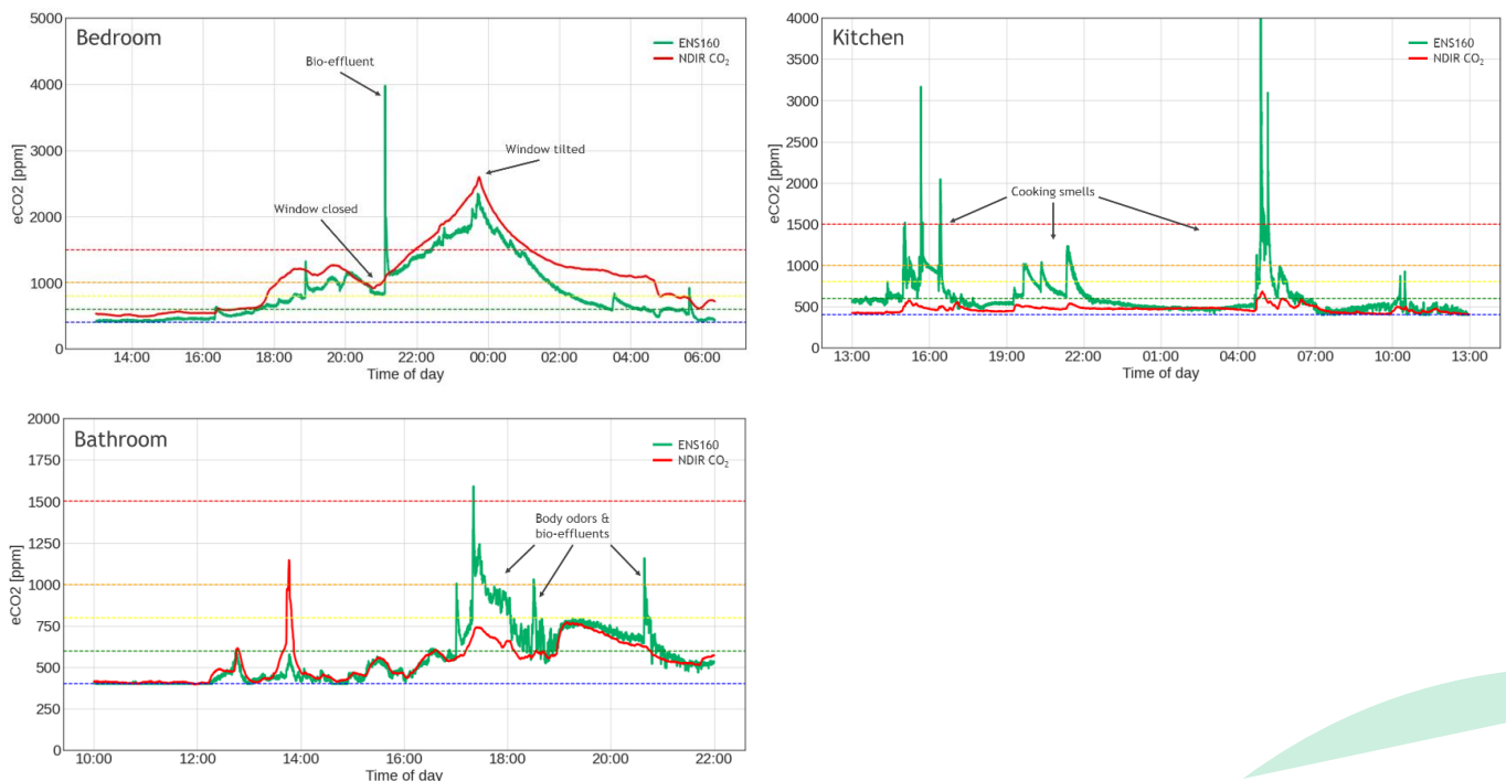
Figure 4: Added value of ENS161's eCO 2 outputs and typical cases of pure CO 2 sensors failing
