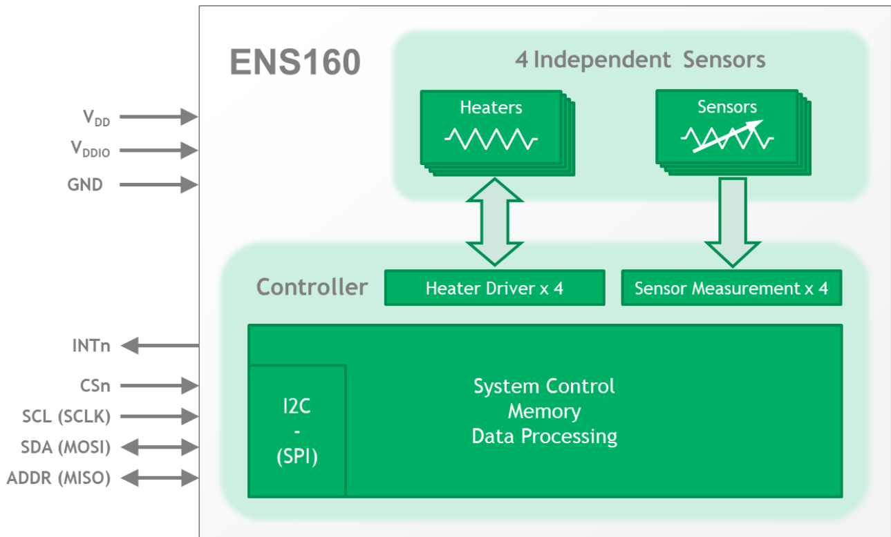
Figure 1: Functional Blocks
