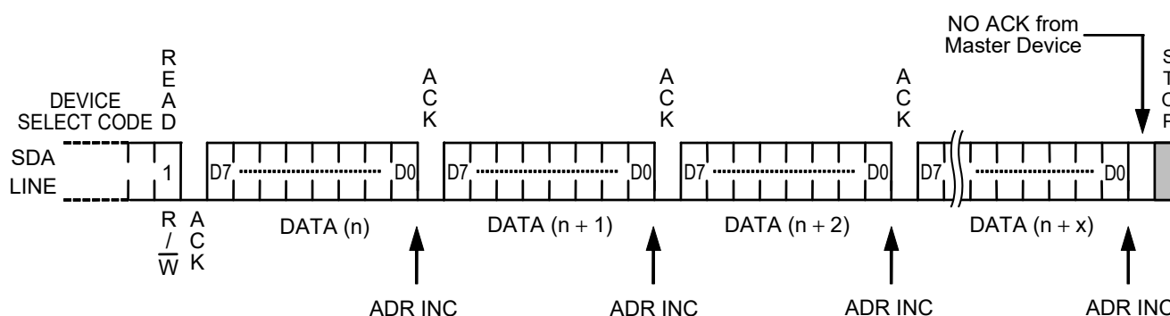
Figure 15 Sequential Read
