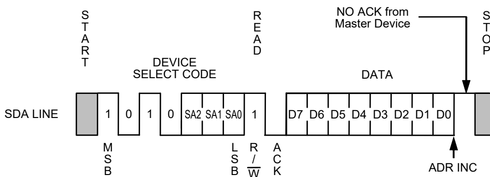
Figure 13 Current Address Read
