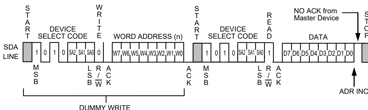
Figure 13 Random Read
