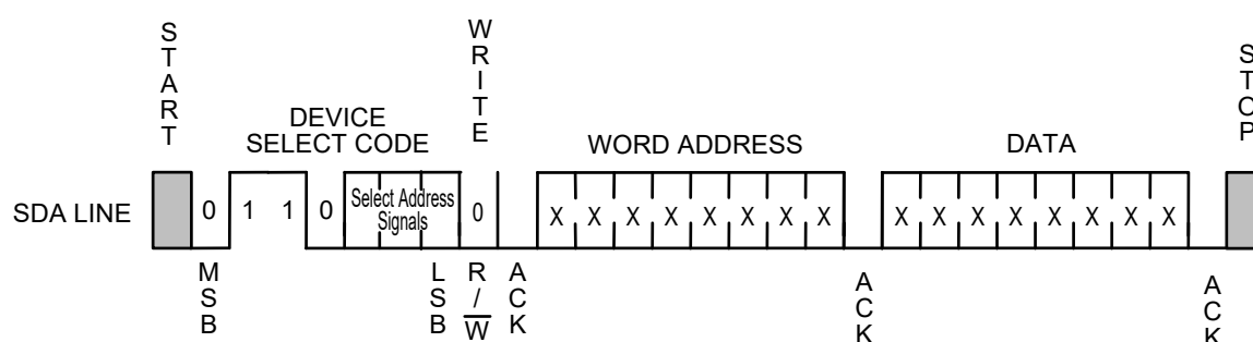
Figure 10 Software Write Protect
