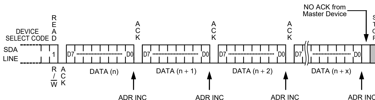
Figure 14 Sequential Read
