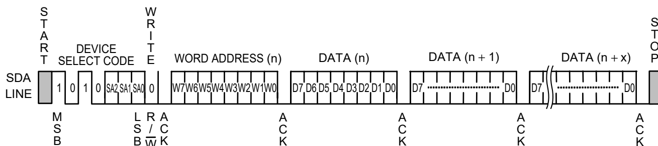
Figure 9 Page Write
