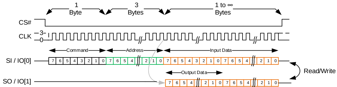
Figure 10: Description of (1-1-1) Instruction Type (Without XIP)
