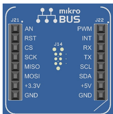
Figure 14. mikroBUS Connection
