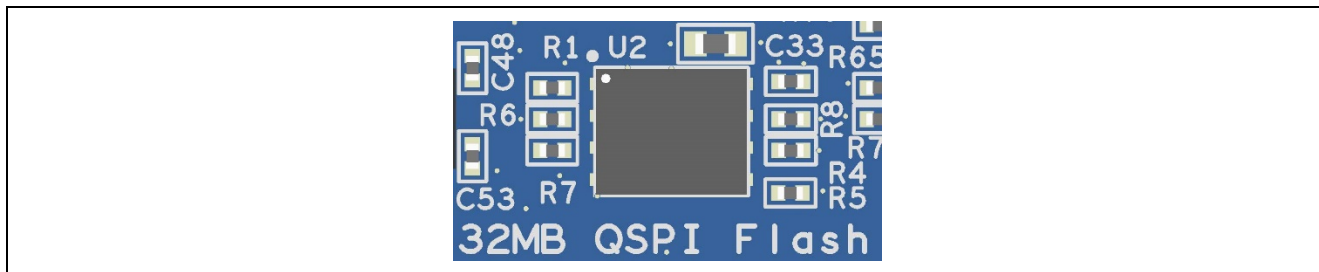
Figure 23. Quad-SPI Flash
