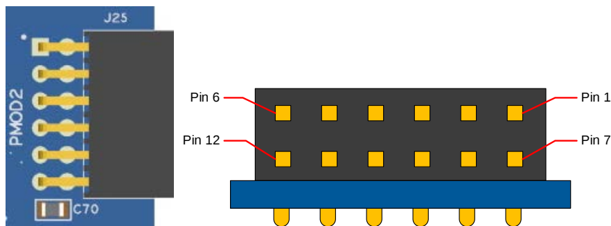
Figure 12. Pmod 2
