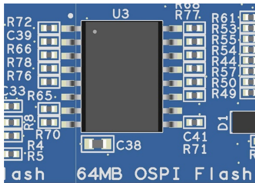
Figure 24. Octo-SPI Flash
