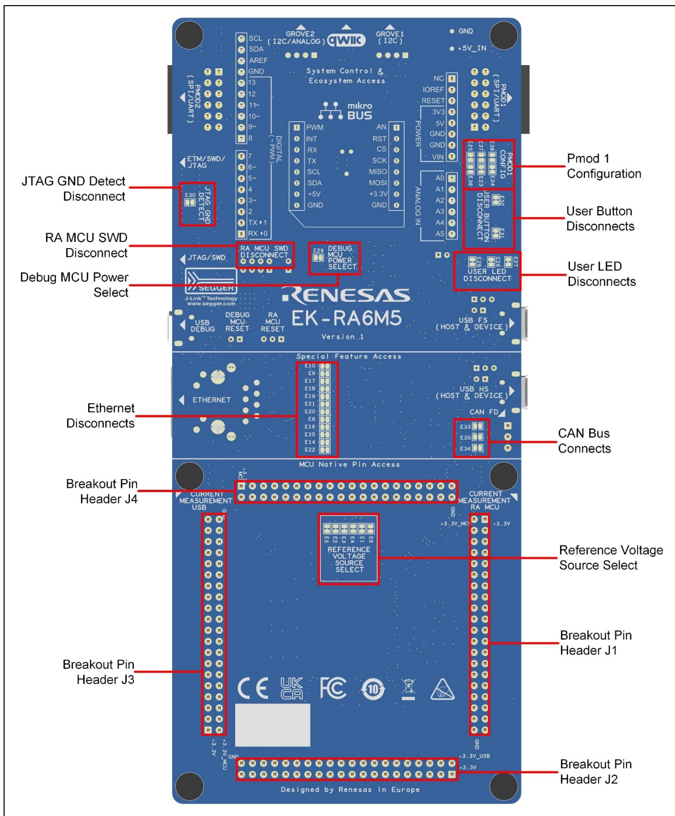
Figure 2. EK-RA6M5 Board Bottom Side
