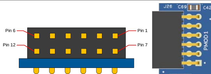
Figure 11. Pmod 1
