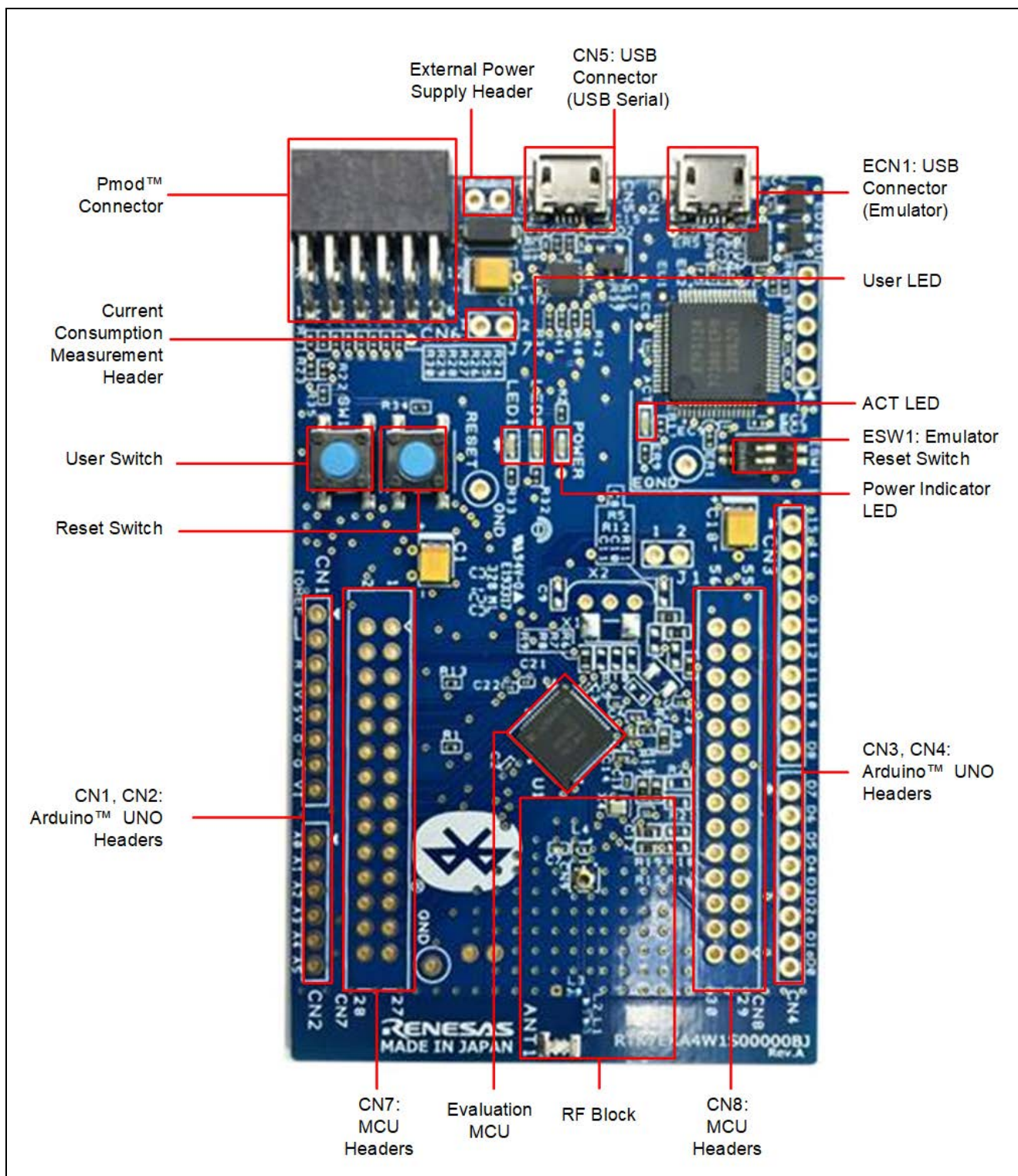
Figure 1. EK-RA4W1 Top Side
