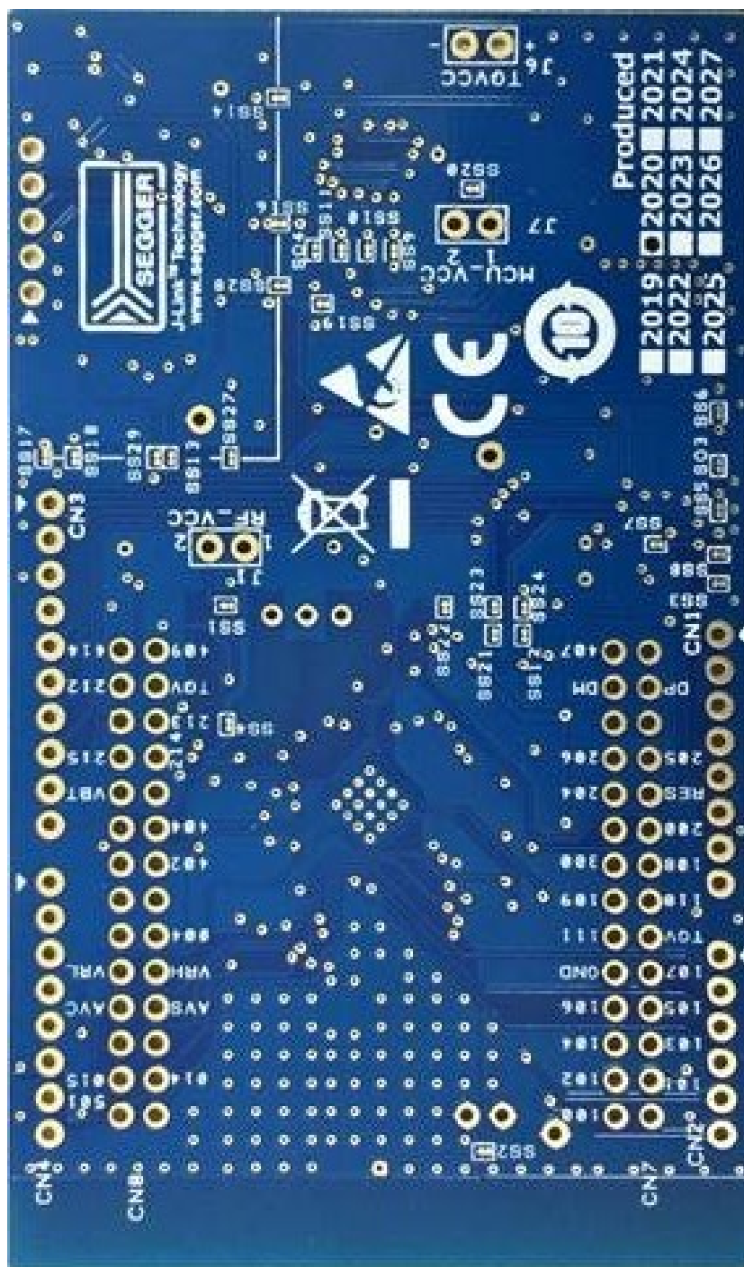
Figure 2. EK-RA4W1 Bottom Side
