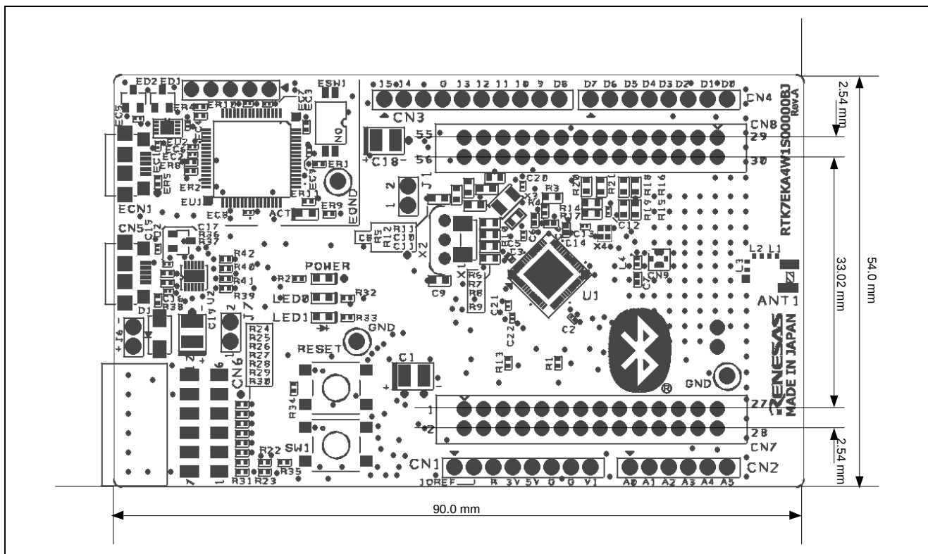
Figure 5. Parts Layout
