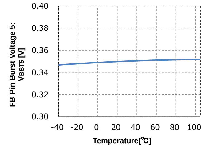
Figure 28. FB Pin Burst Voltage 5 vs Temperature
