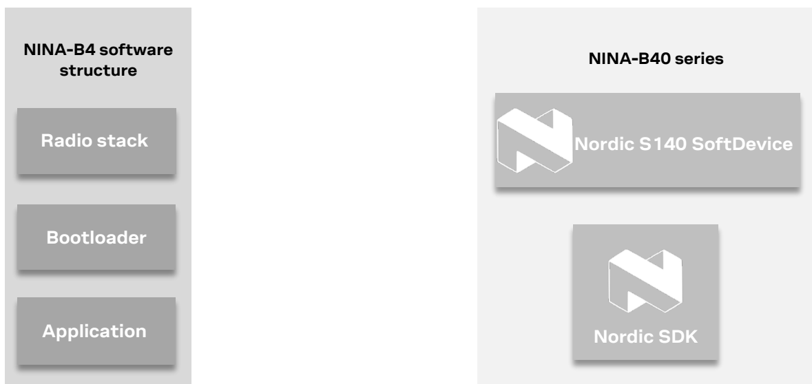
Figure 2: NINA-B40 software structure and available software options
