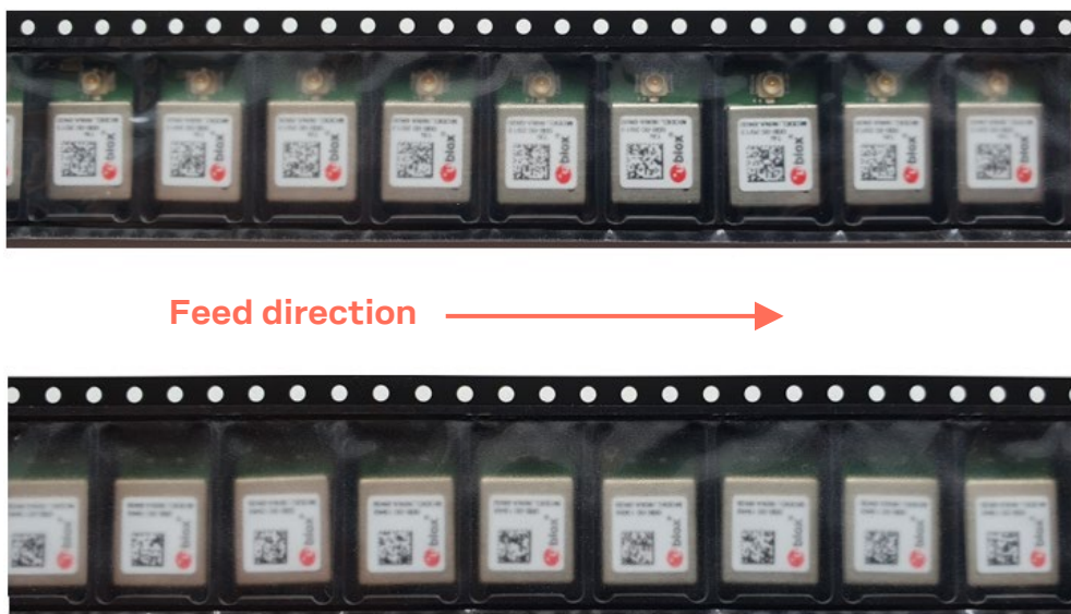
Figure 7: Orientation of NINA-B4 modules on tape representing the same orientation for NINA-B40 modules
