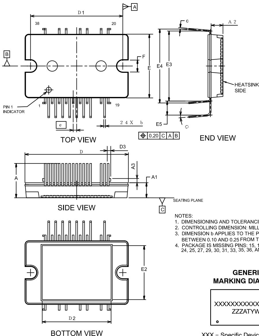
DIP38 29.60x18.20 EP-5 CASE 181AE ISSUE A
