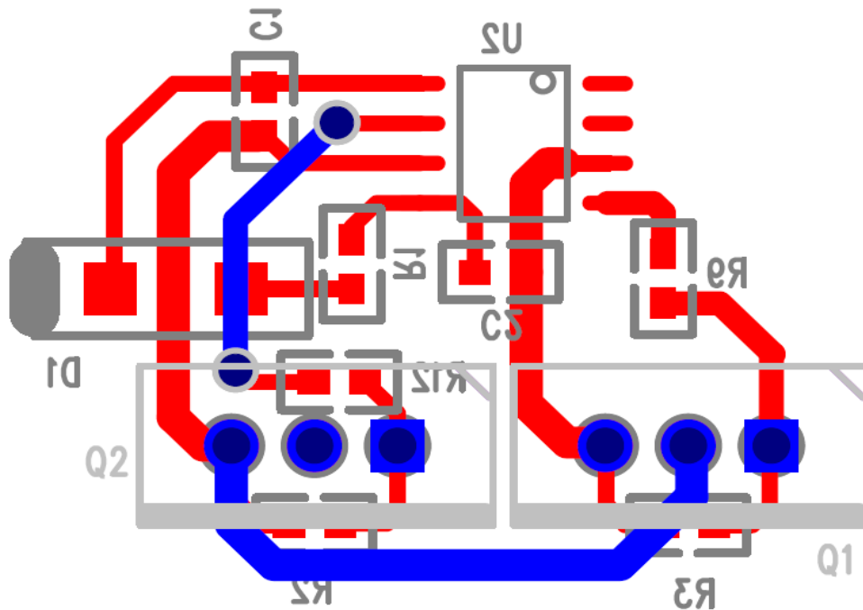
Figure 35. Example Layout
