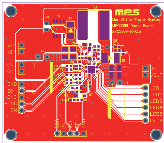
Figure 3: Top Layer
