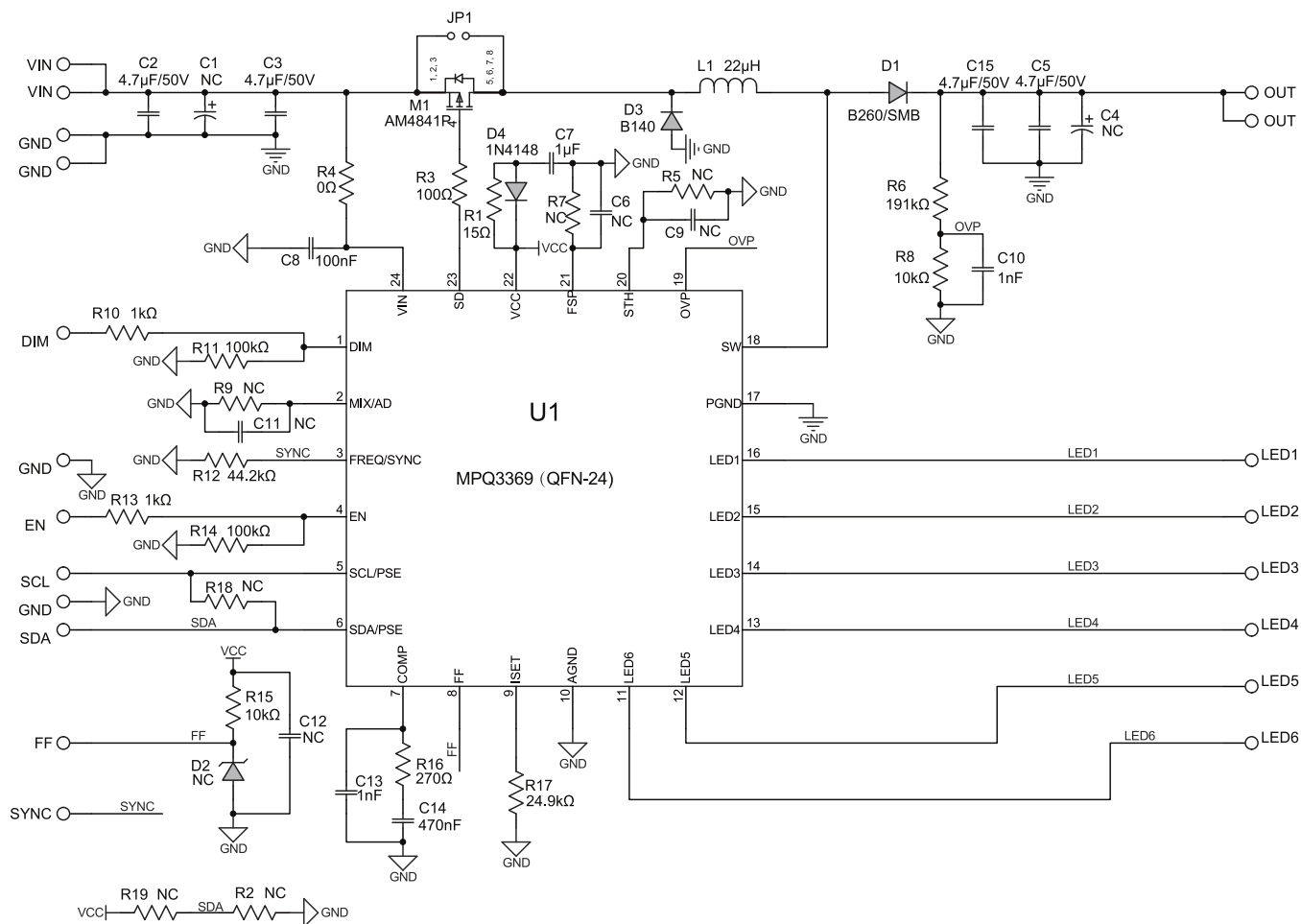
Figure 2: Evalutation Board Schematic
