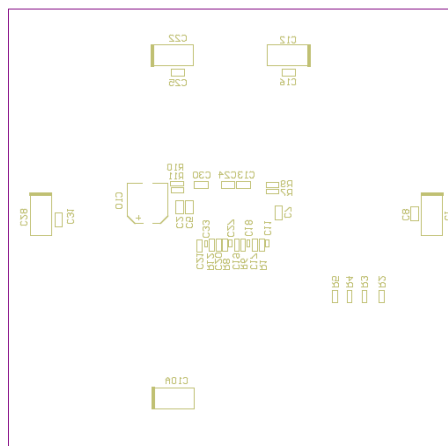
Figure 9: Bottom Silk
