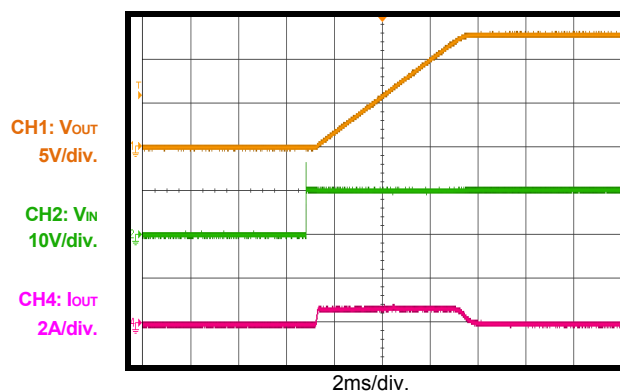
Start-Up through Input Voltage I_{OUT}=0A , C_{OUT}=1000\mu F
