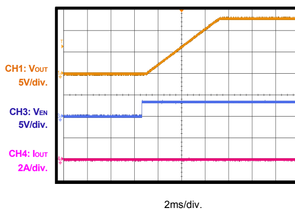
Start-Up through Enable I_{OUT}=0A
