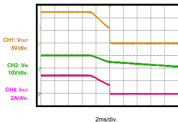
Shutdown through Input Voltage I_{OUT}=3A
