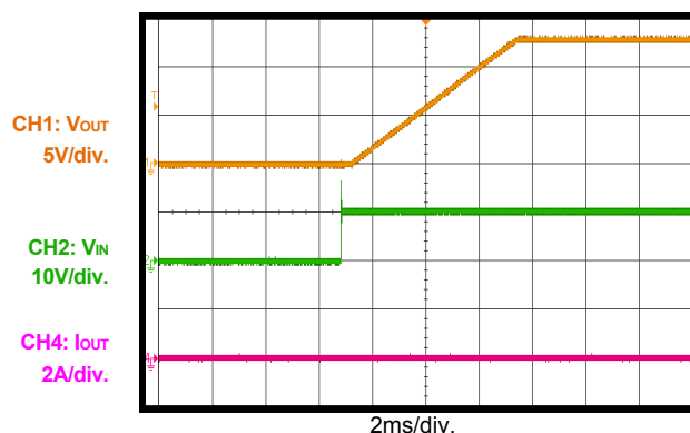
Start-Up through Input Voltage I_{OUT}=0A
