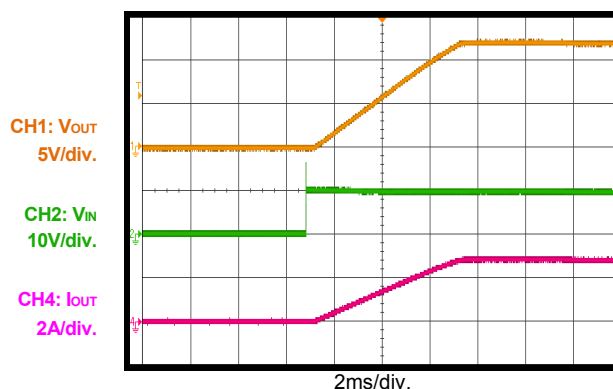
Start-Up through Input Voltage I_{OUT}=3A
