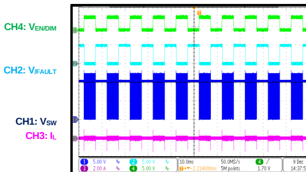
PWM Dimming
