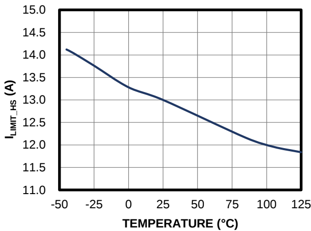
HS Current Limit vs. Temperature
