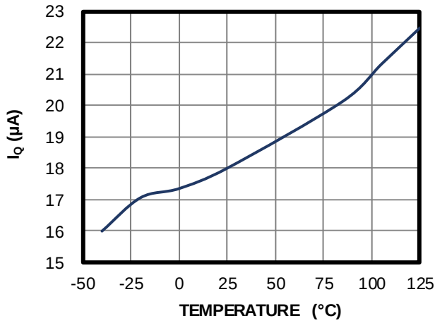
V_{IN} Quiescent Current vs. Temperature
