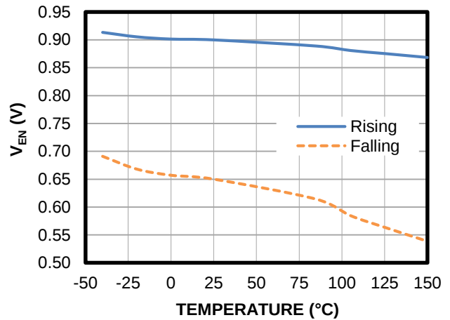
V_{EN} Rising and Falling Threshold vs. Temperature
