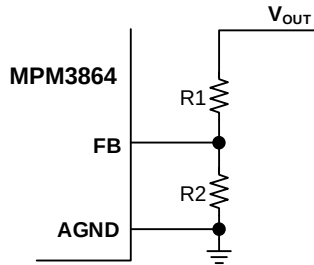
Figure 5: Feedback Network
