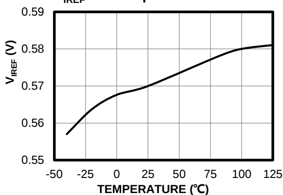
V_{IREF} vs. Temperature
