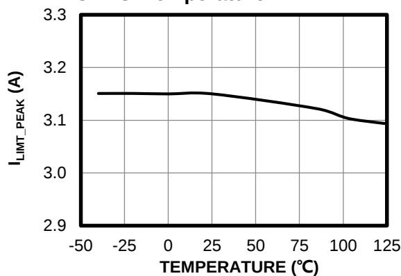
Current Limit with MOSFETs Half On vs. Temperature
