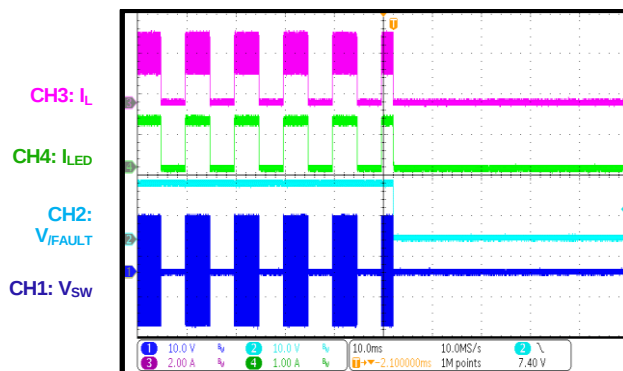
IREF Open Fault after IC Starts Up PWM dimming
