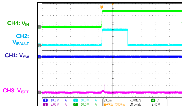
ISET Open Fault before IC Starts Up
