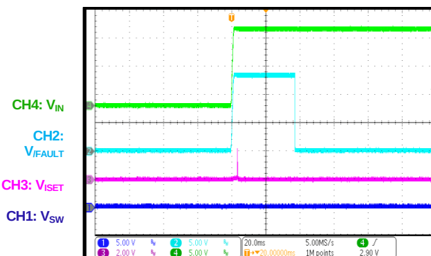
ISET Open Fault before IC Starts Up
