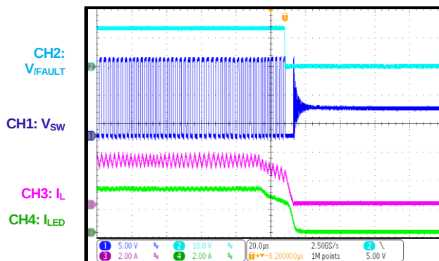
ISET Open Fault after IC Starts Up
