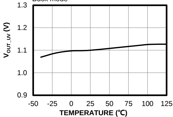
V_{OUT} UV Threshold vs. Temperature Buck mode
