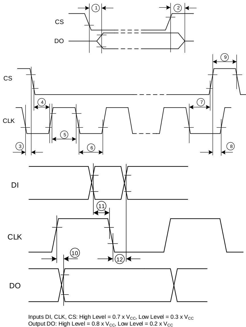
Figure 1: Serial Interface Timing Diagram
