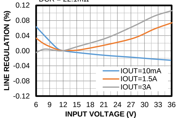
Line Regulation
