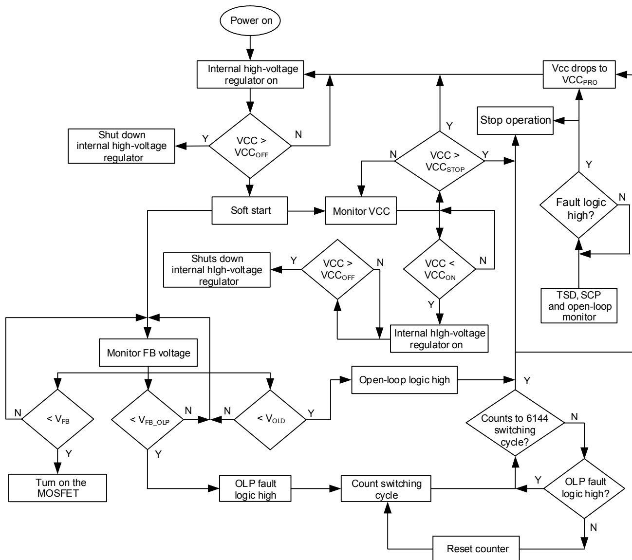
Figure 11: Control Flowchart
