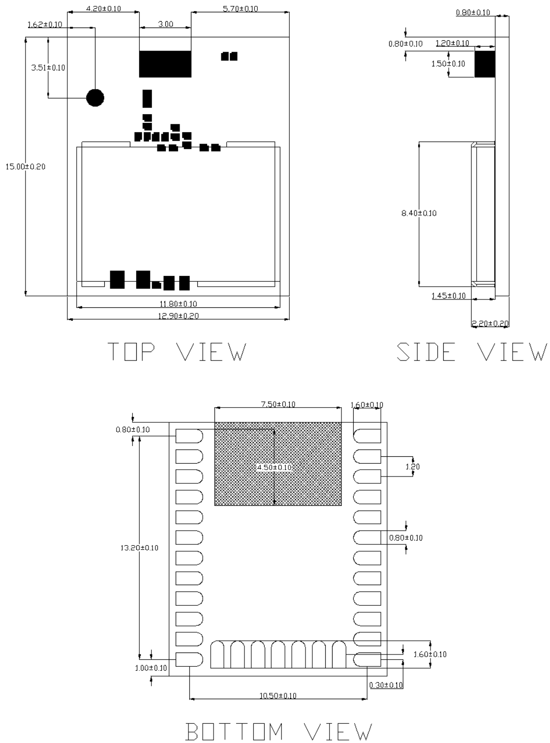
Figure 8.1. Module Dimensions
