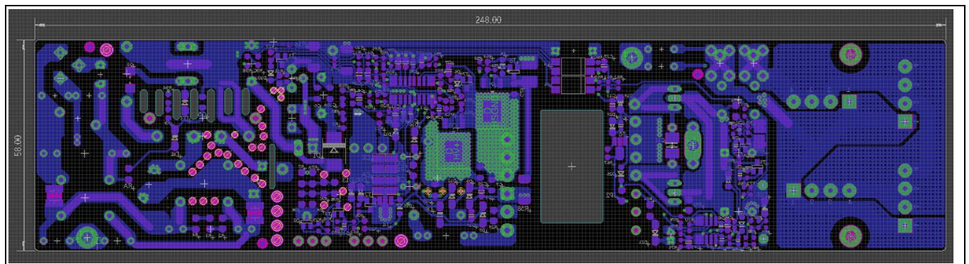
Figure 8 ICL5102 320 W reference design – PCB bottom side
