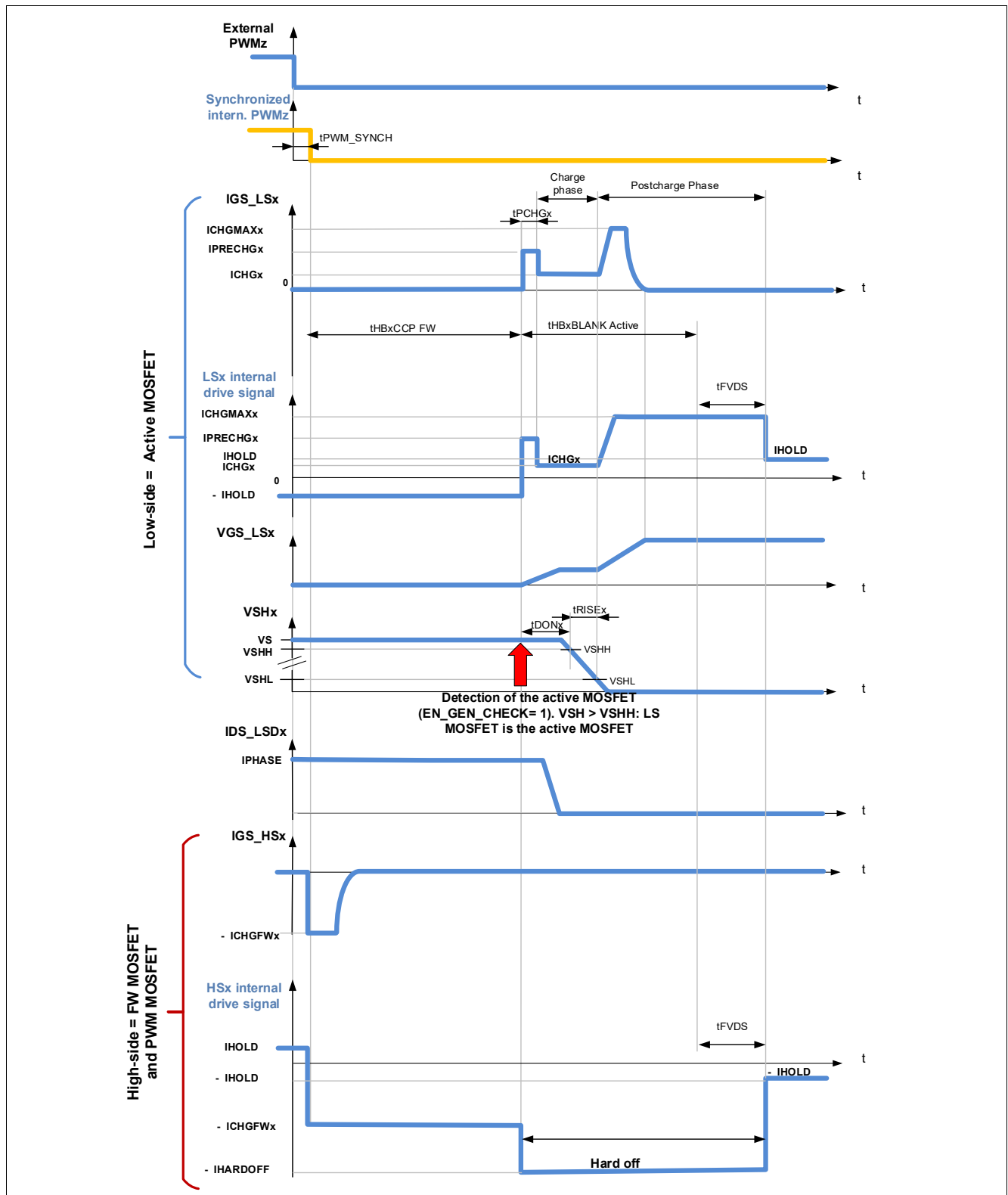
Figure 52 PWM falling edge - PWM mode with active gate control, HS PWM (HBxMODE = 10 B ) , LS as active MOSFET, HS as FW MOSFET. PWM_NB = 0 (one PWM input per HB), AGC = 01 B or 10 B (Active Gate Control), EN_GEN_CHECK = 1 (detection of active / FW MOSFET), AFWx = 1 (active freewheeling for HBx is activated)
