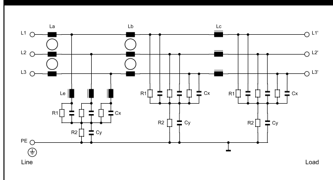
FN3271 typical electrical schematic (>100 A)
