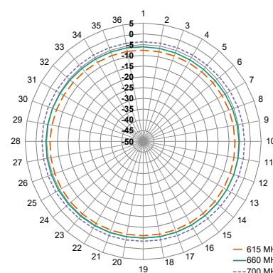
XY-Plane Gain
