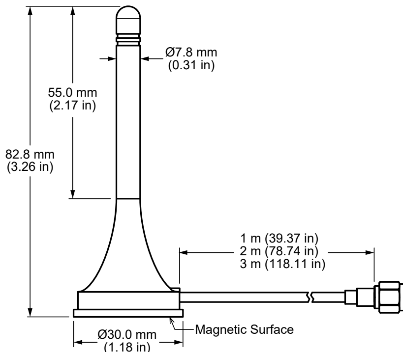
Figure 1. ANT-5GW-MMG1-SMA Series Antenna Dimensions
