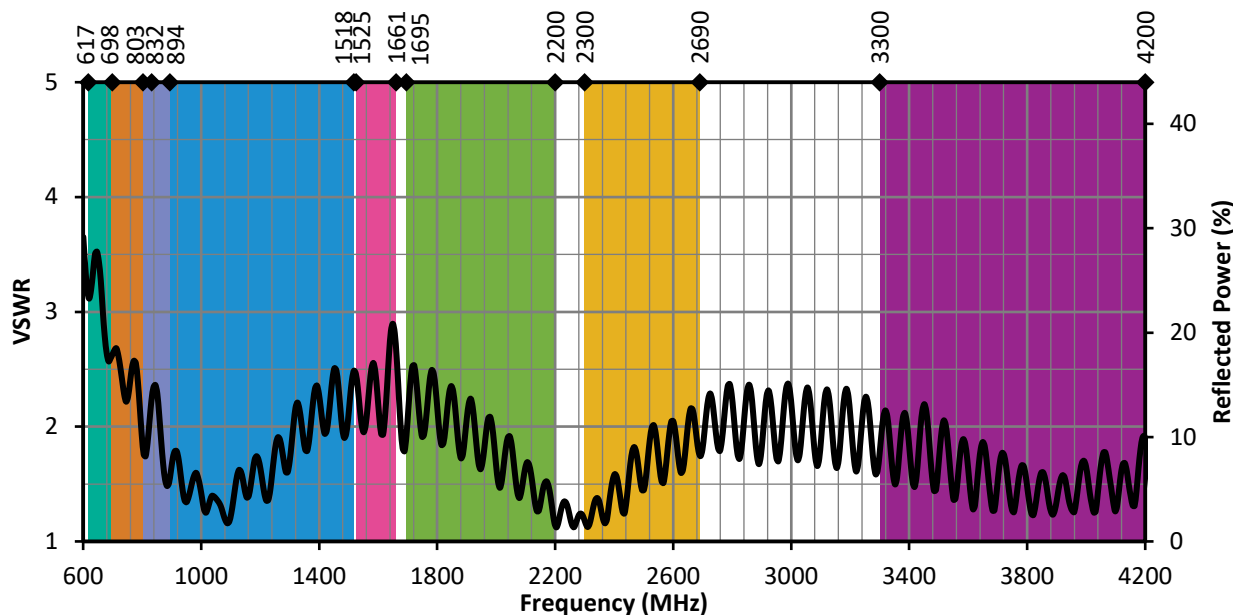
Figure 11. ANT-5GW-MMG1-SMA VSWR, Free Space
