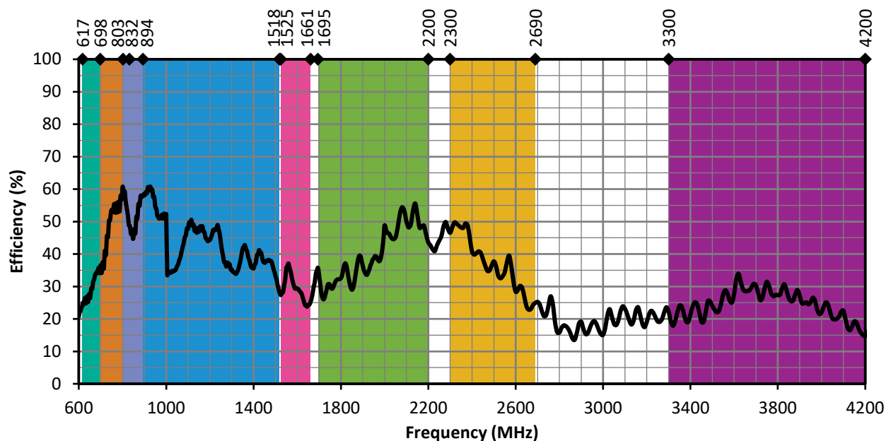
Figure 15. ANT-5GW-MMG1-SMA Antenna Efficiency, Free Space
