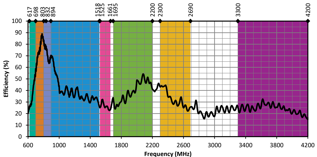
Figure 8. ANT-5GW-MMG1-SMA Antenna Efficiency on Ground Plane
