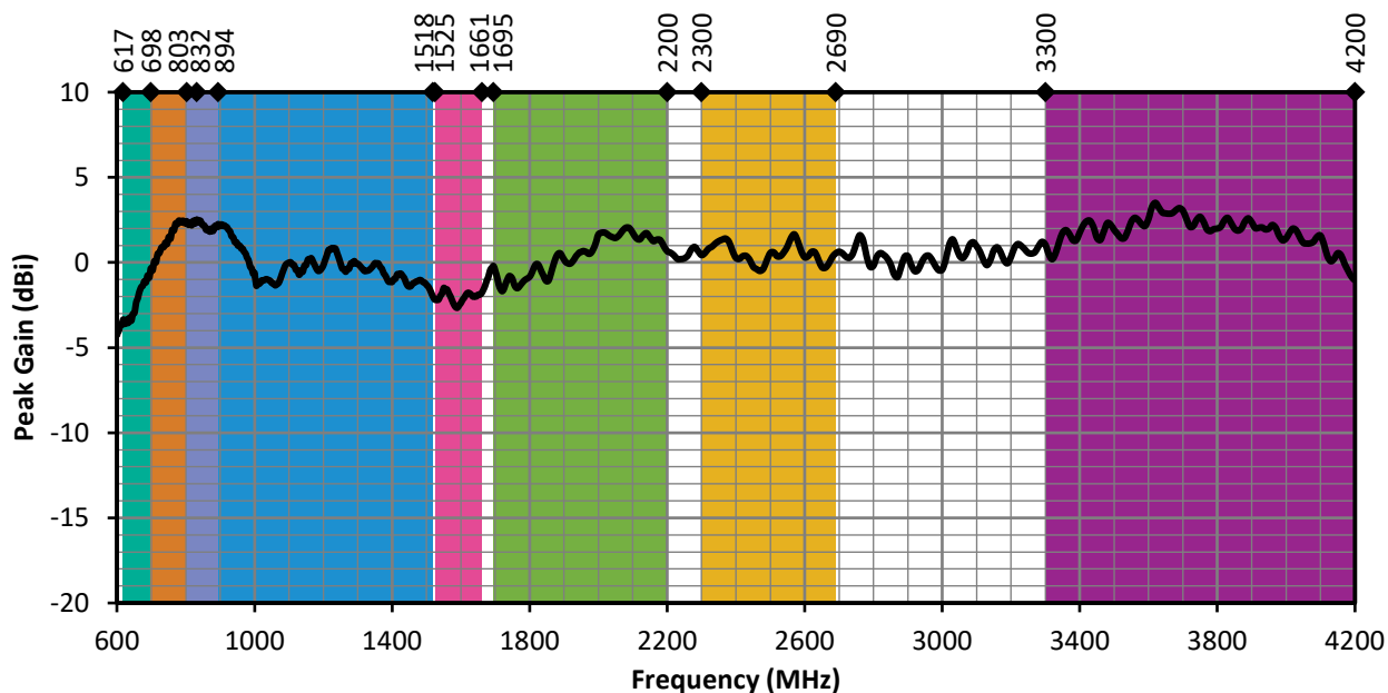
Figure 6. ANT-5GW-MMG1-SMA Peak Gain on Ground Plane
