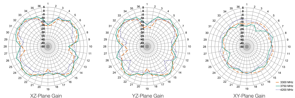
Figure 16. ANT-5GW-MMG1-SMA Radiation Patterns in Free Space
