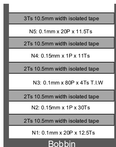
Figure 7: Winding Diagram
