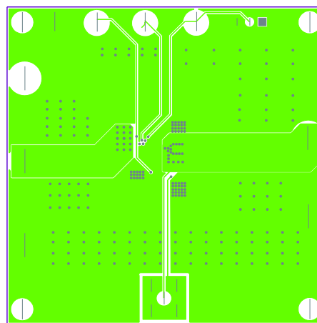
Figure 4: Mid-Layer 2
