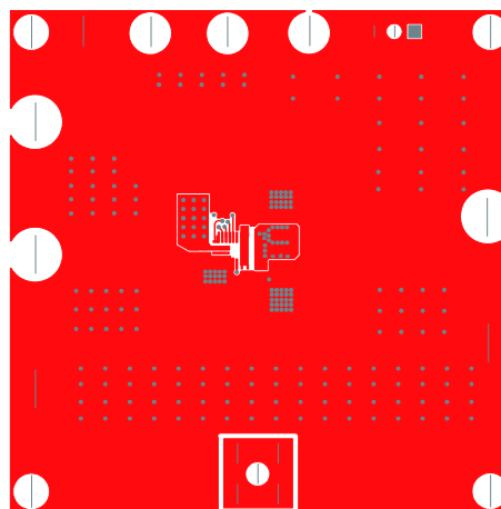
Figure 2: Top Layer
