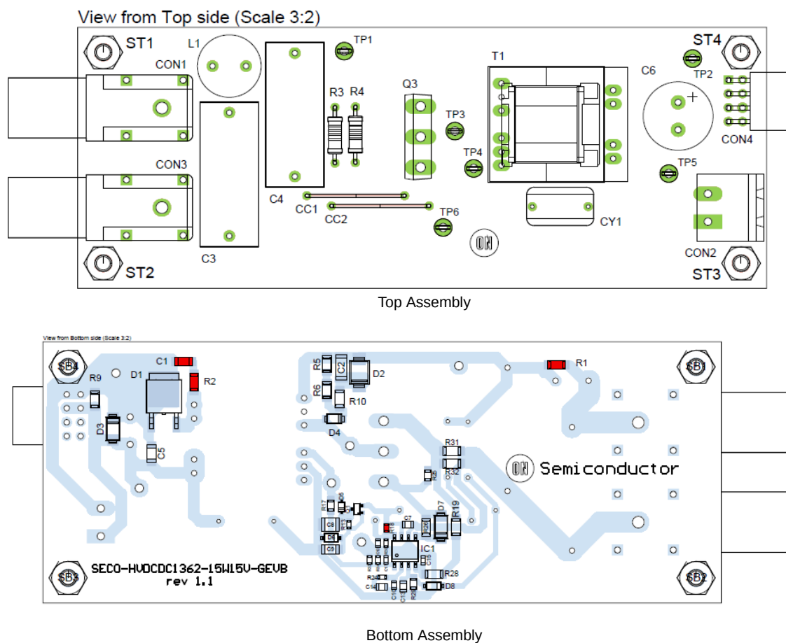
Figure 22. Layout
