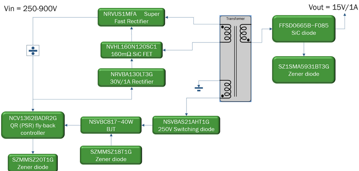
Figure 3. Block Diagram
