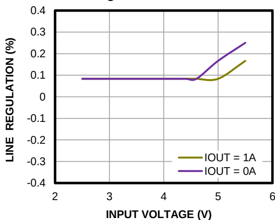
Line Regulation
