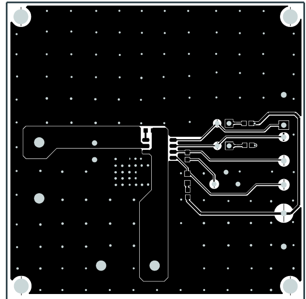
Figure 3: Top Layer
