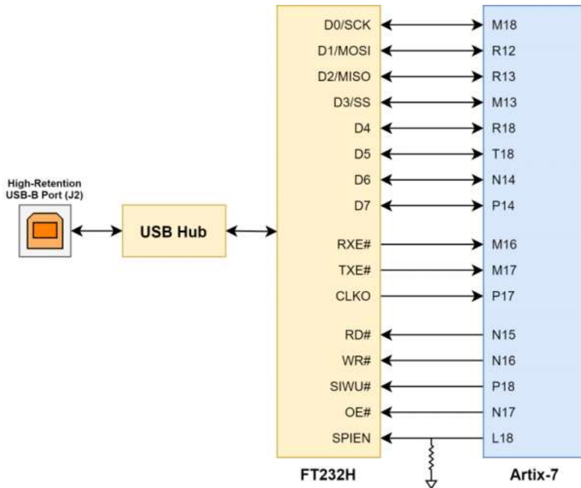
Figure 6.1.1 USB104 A7 DPTI Connections
