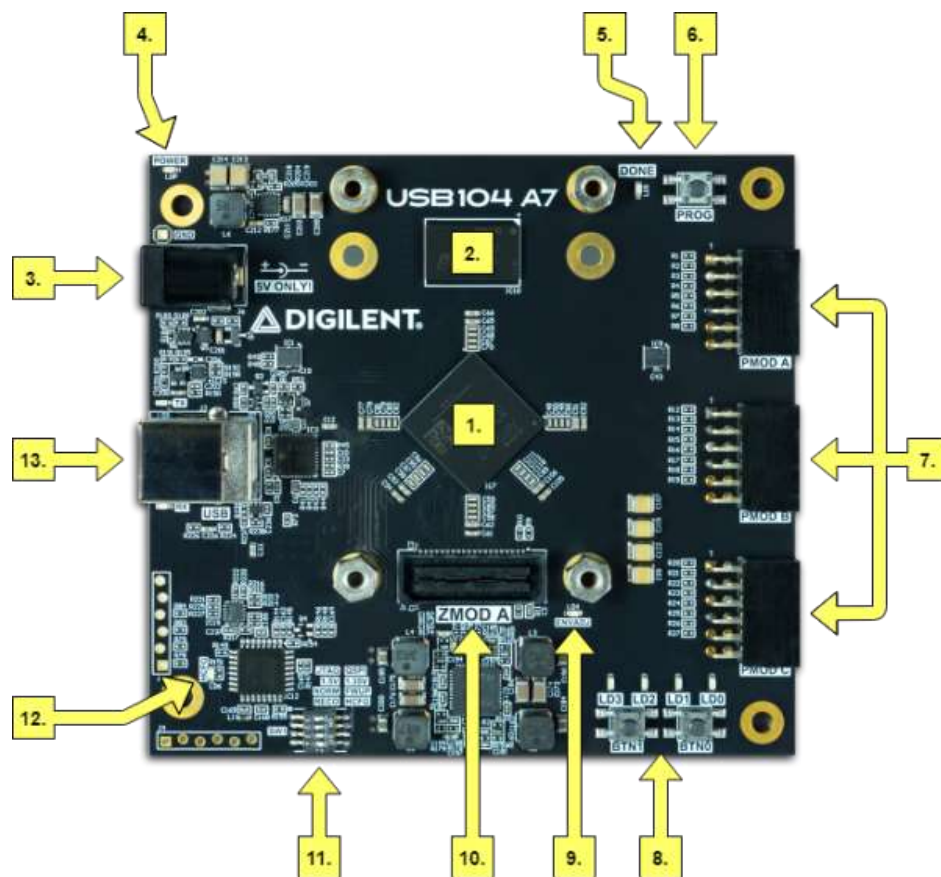
USB104 A7 Callout Diagram
