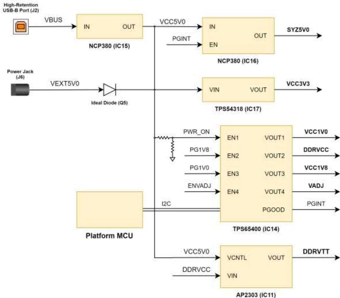
Figure 1.1: Power Circuit Overview
