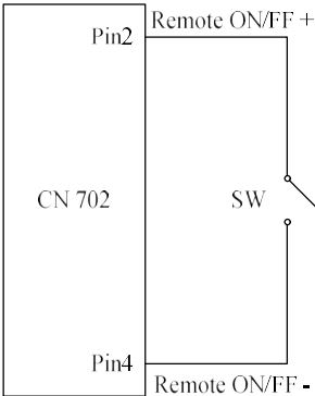
Figure 7. Remote On/Off Connection
