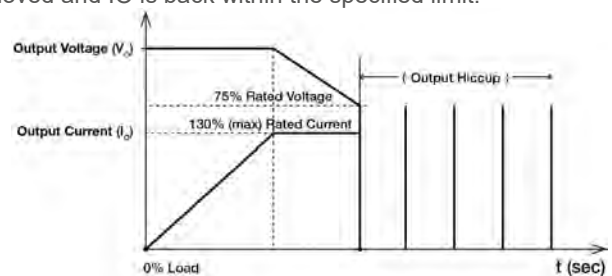
Figure 6. Hiccup at OLP/OCP
