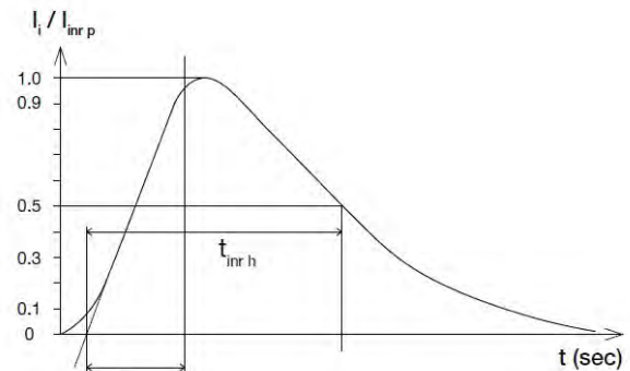
Figure 5. Inrush Current
