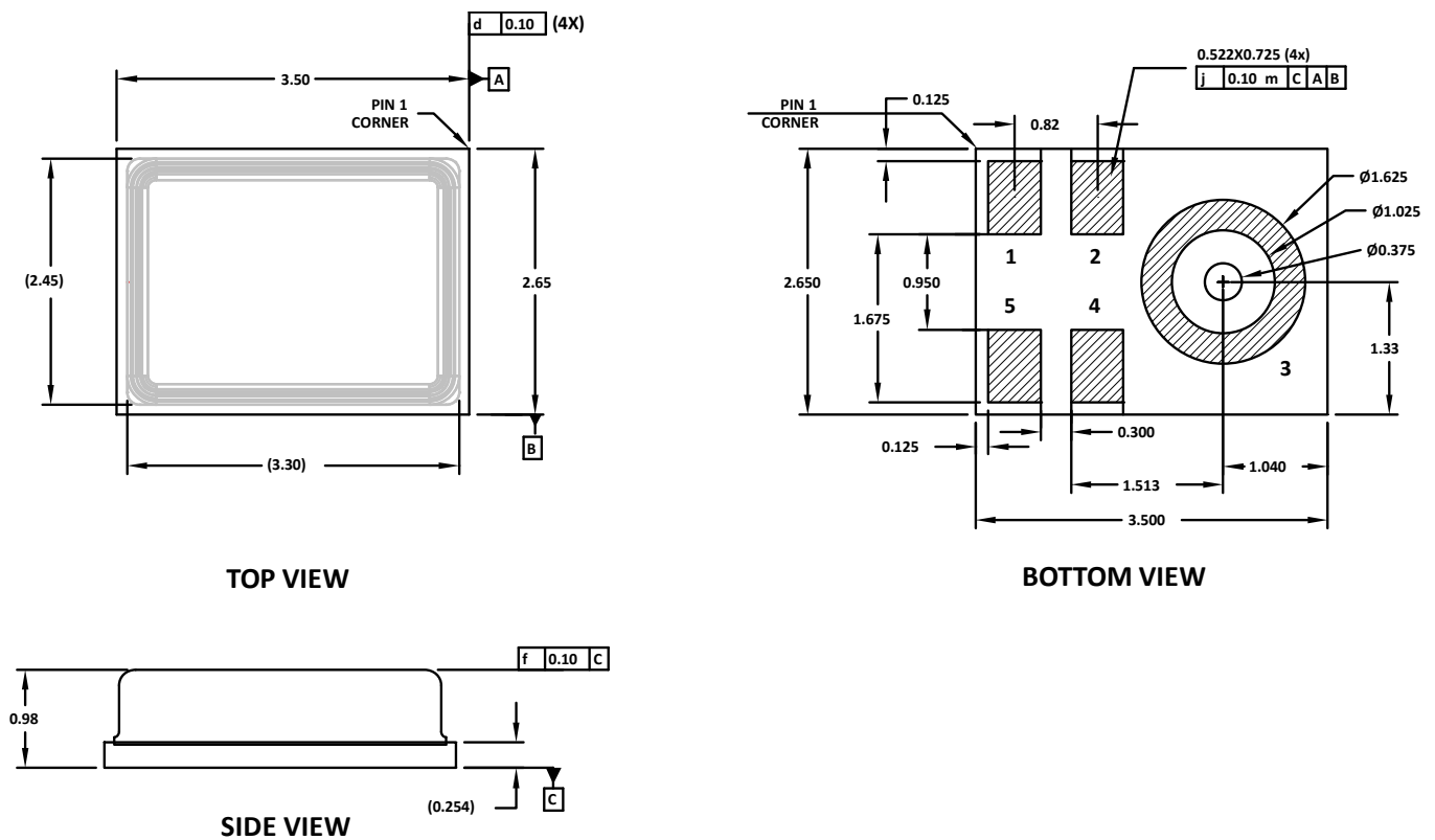
Figure 11. 5-Terminal Chip Array Small Outline No Lead Cavity 3.50 mm × 2.65 mm × 0.98 mm Body Dimensions shown in millimeters
