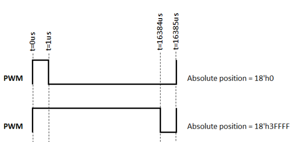
PWM Period: 16385 \mu s
