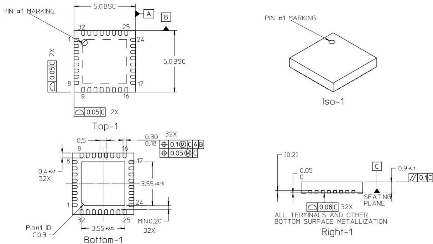
Figure 5: AEAT-9955, 32 QFN Dimensions
