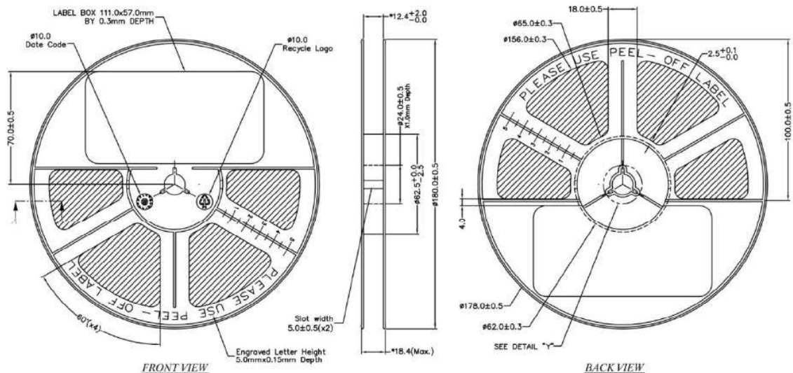
Figure 6: Reel Dimensions
