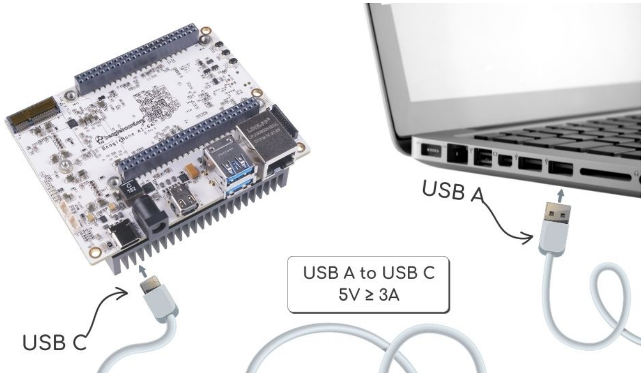
Figure 3. Tethered Configuration
