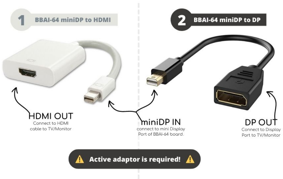
Figure 10. Display adaptors
