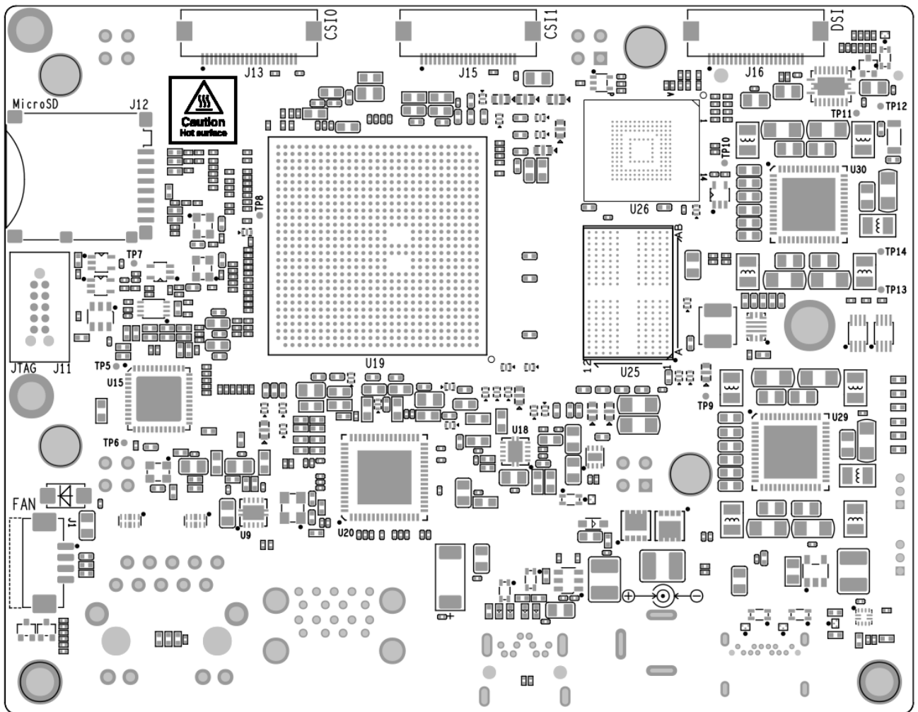
Figure 21. Top silkscreen
